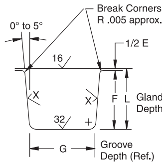
Dynamic Gland
