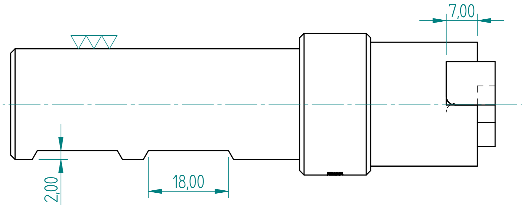
D28 O Ring Groove Bar FOR MACHINING O-RING GROOVE ON FLAT FACE IN CAST IRON
