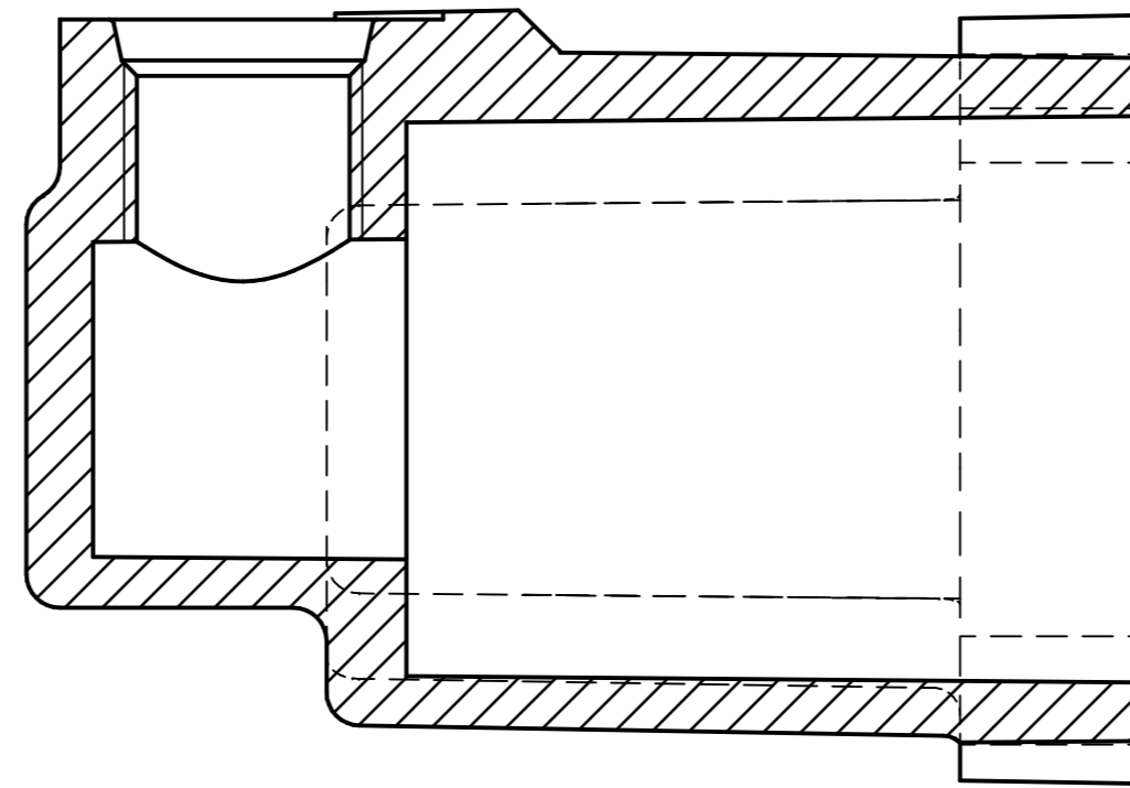
SECTION C-C
