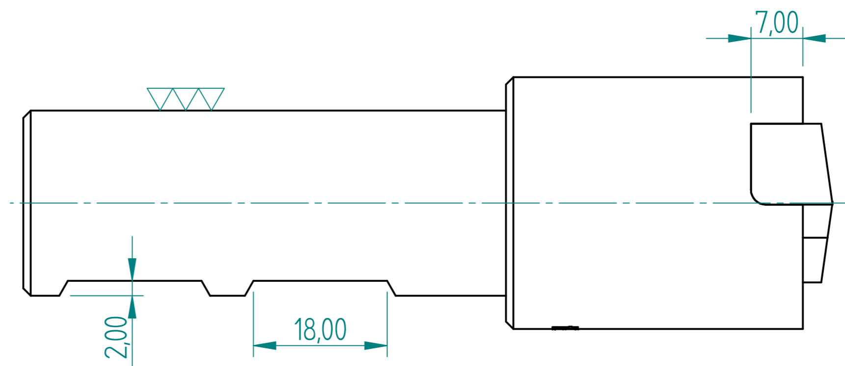
D34 O Ring Groove Bar FOR MACHINING O-RING GROOVE ON FLAT FACE IN CAST IRON 2.1 mm DEEP
