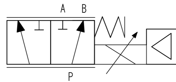
PROPORTIONAL VALVE INTEGRATED AMPLIFIER
