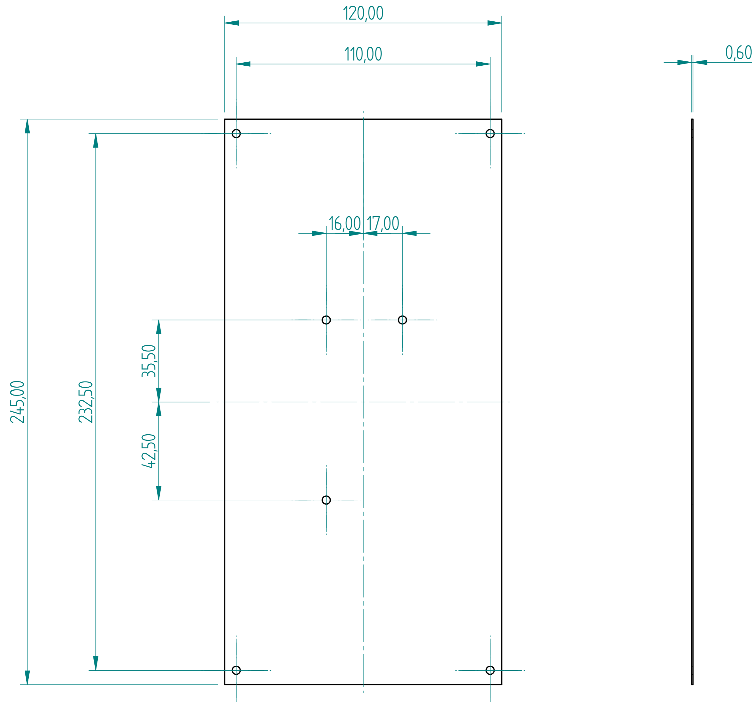
MOUNTING PLATE
