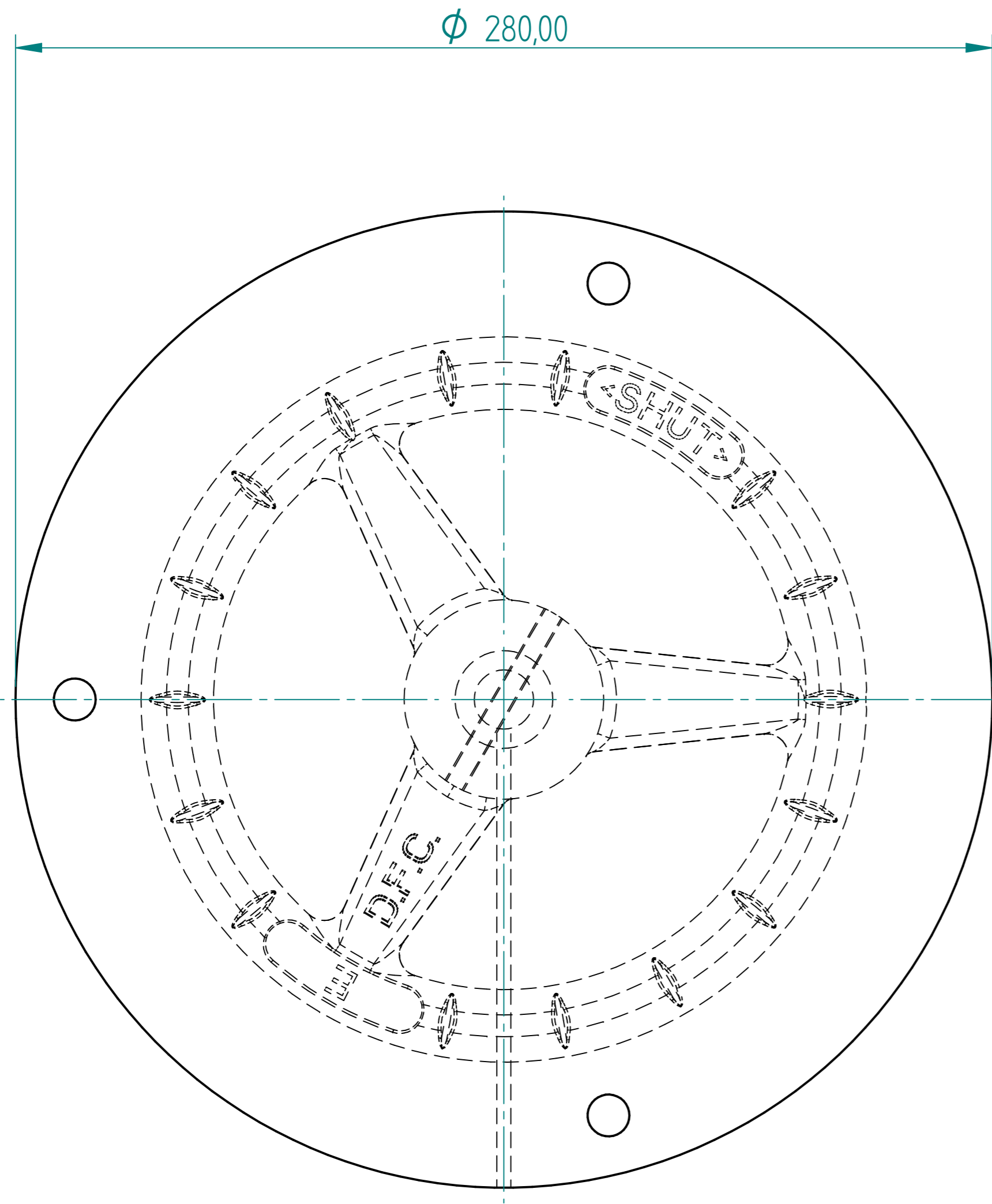
IH200RDS Mould
