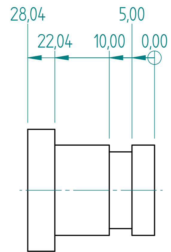
Core Pin
