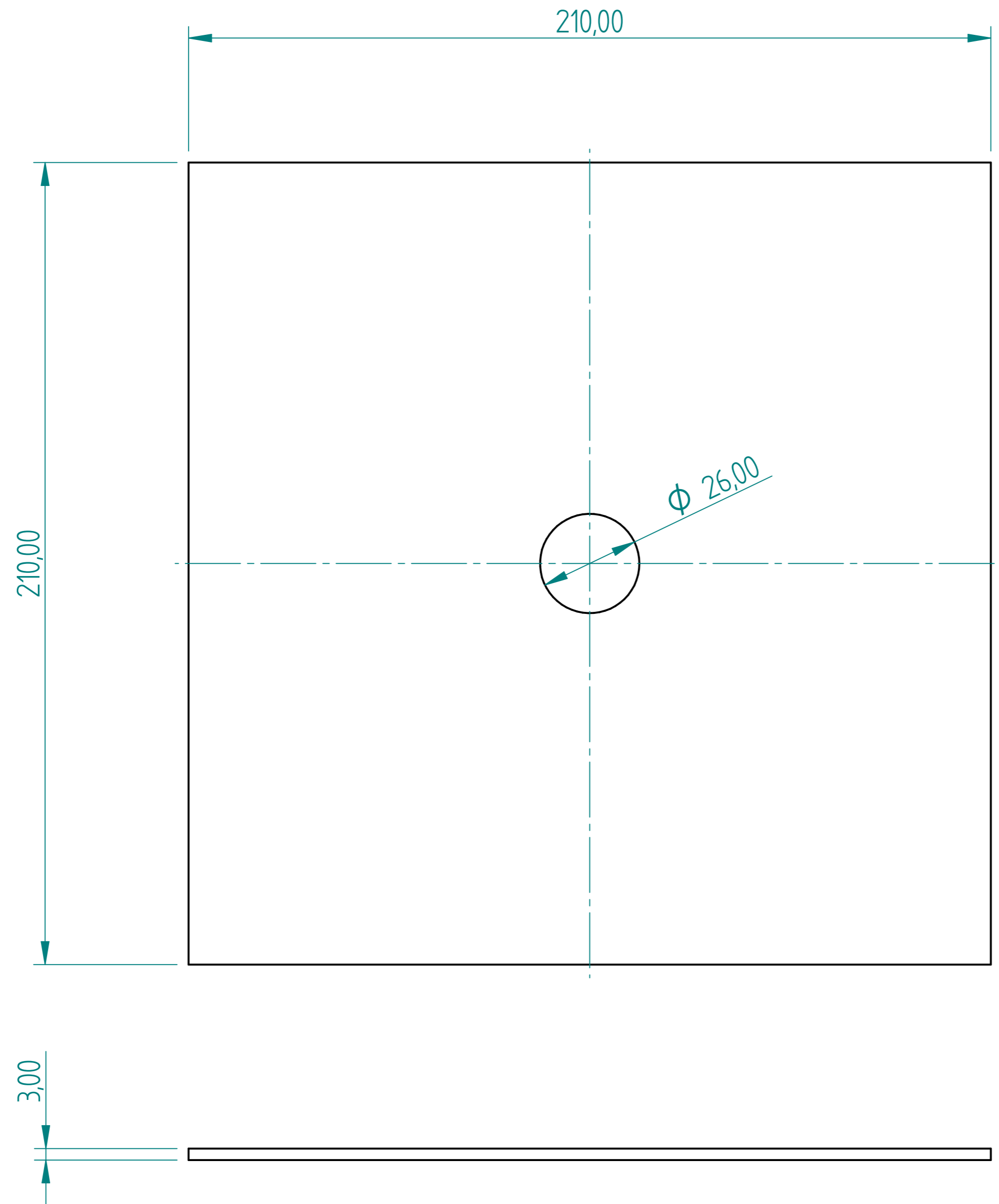
Base Plate
