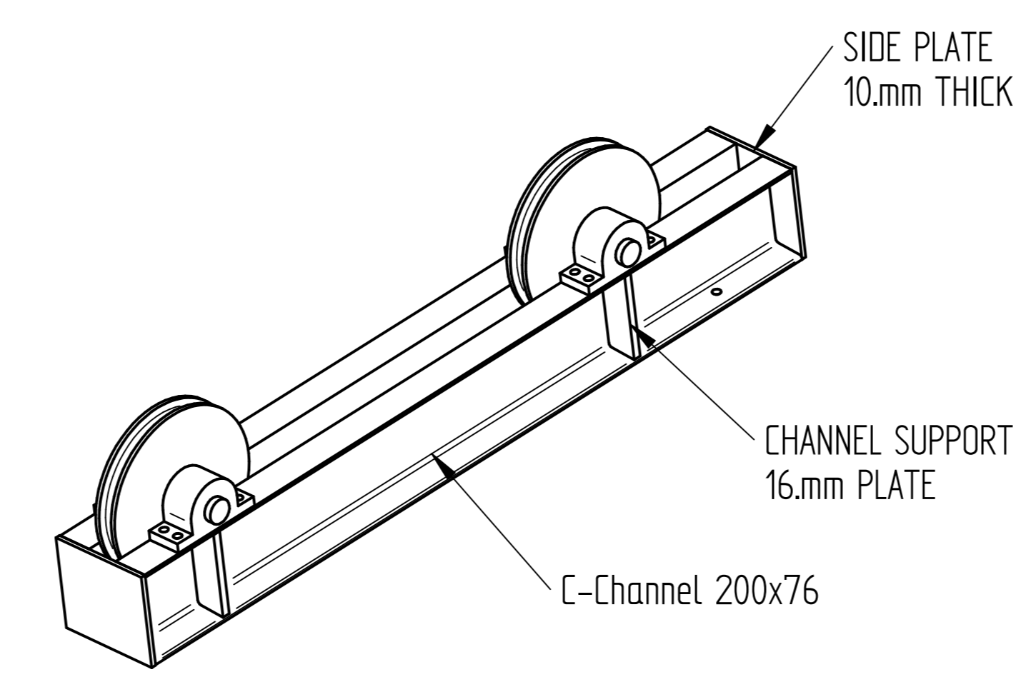
SHEAVE WHEEL BRACKET
