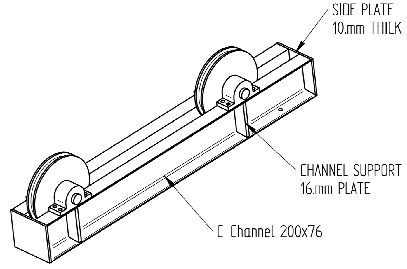
SHEAVE WHEEL BRACKET
