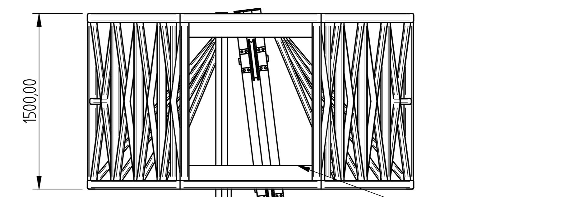
DEAD MAN ARM SHEAVE WHEEL BRACKET
