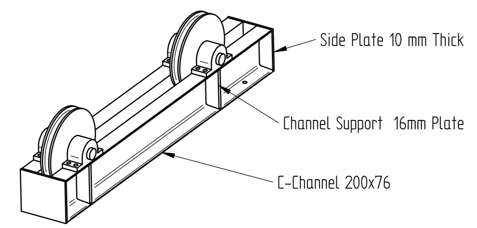
SHEAVE WHEEL BRACKET
