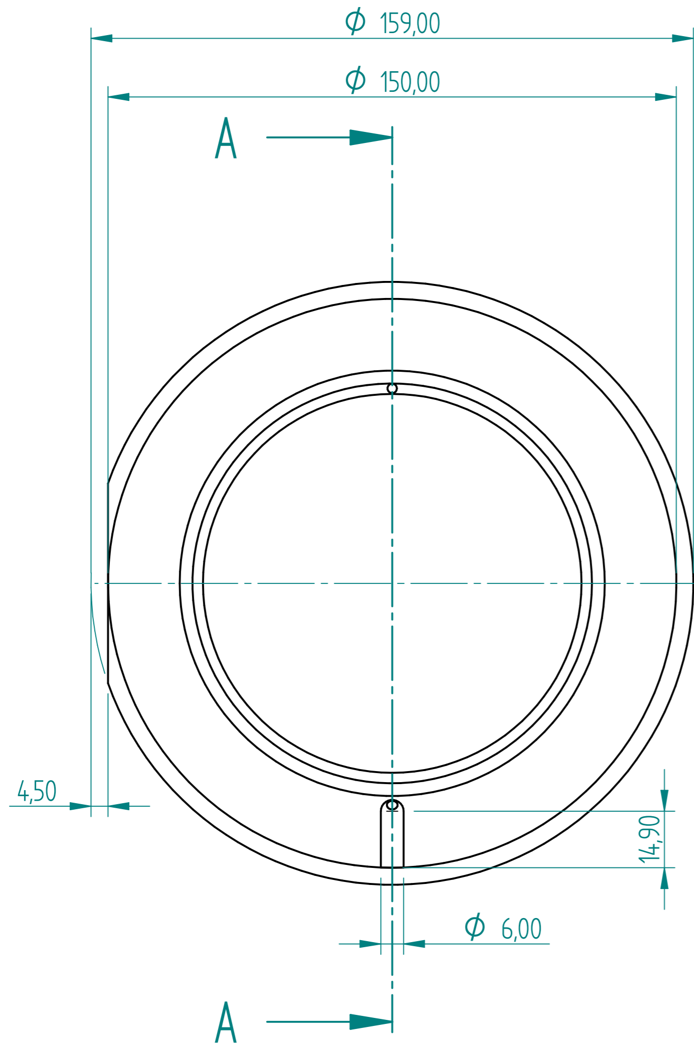
FH Insert A 16 off +25mm
