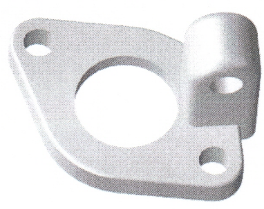
V75 Handle Bracket Part No: 7502 Matl: Zinc 2 95gr
